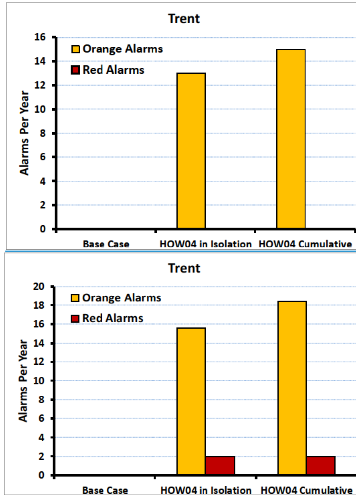
Figure 43: Modelled yearly alarm rates for the Trent platform.
