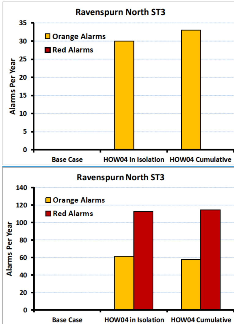
Figure 35: Modelled yearly alarm rates for the Ravenspurn North ST3 platform.
