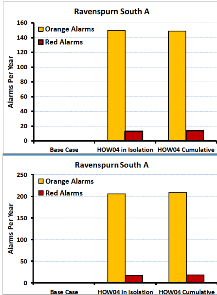
Figure 36: Modelled yearly alarm rates for the Ravenspurn South A platform.
