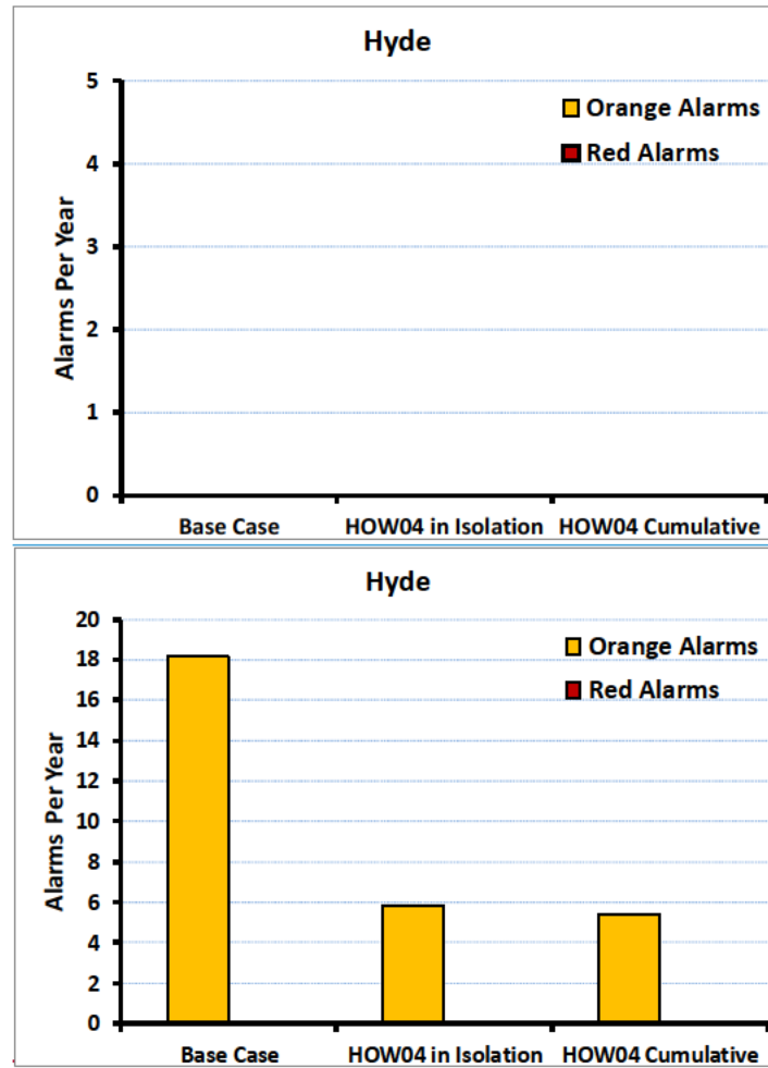
Figure 42: Modelled yearly alarm rates for the Hyde platform.
