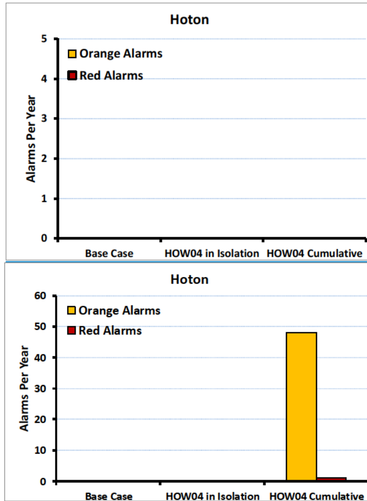
Figure 41: Modelled yearly alarm rates for the Hoton platform.
